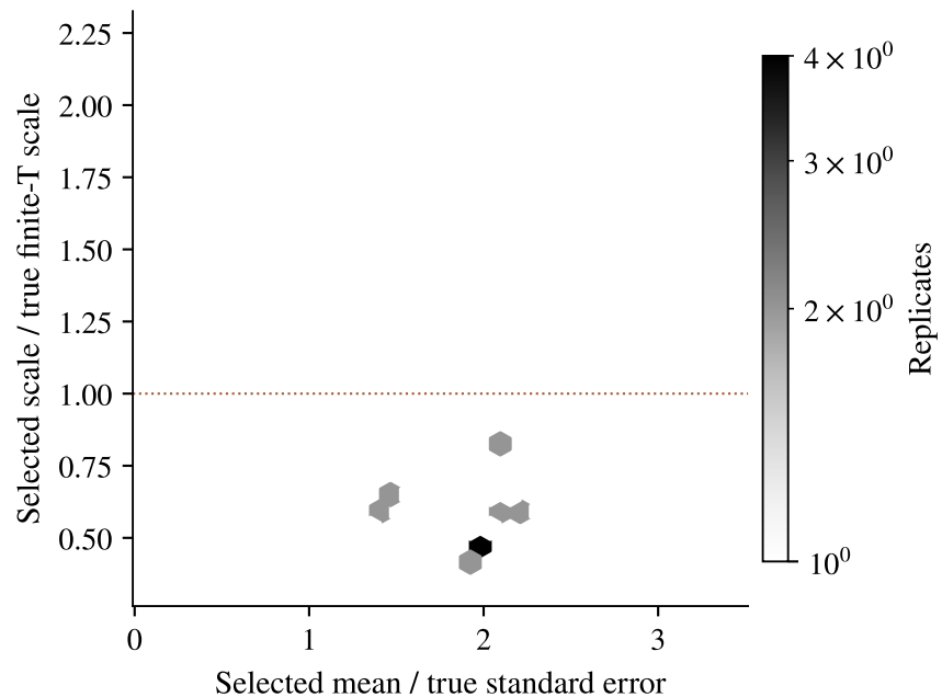
(b) Fitted finite-T tail winner
