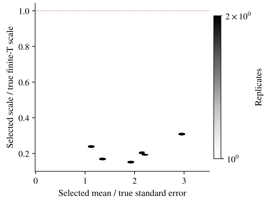
(a) Bartlett winner
