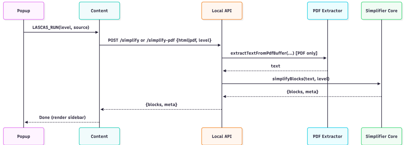
Figure 4: End-to-end request path
