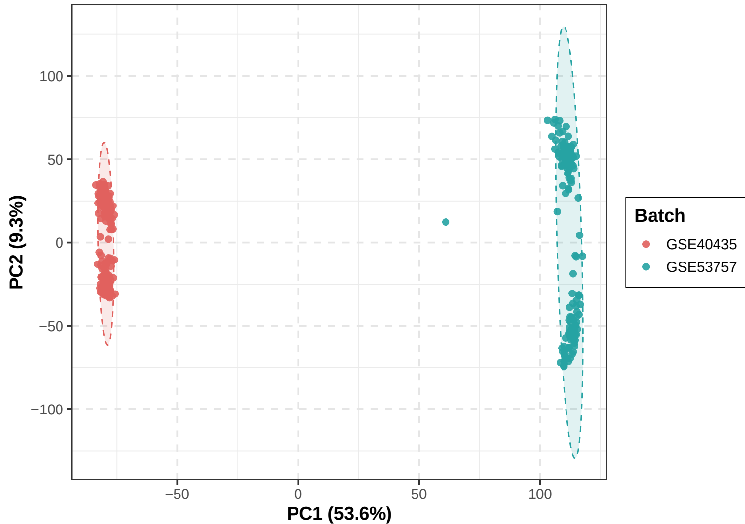
PCA_Before Batch Effect
