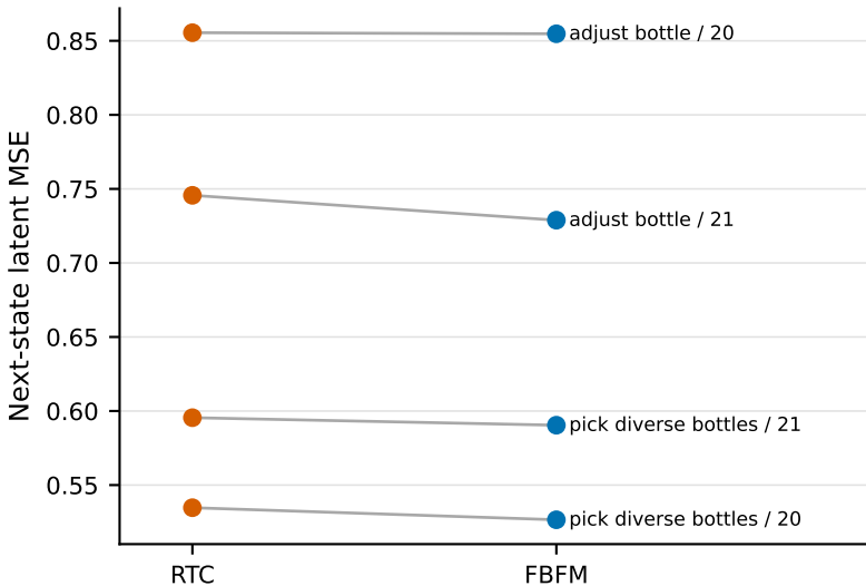
Paired wave-0 state prediction
