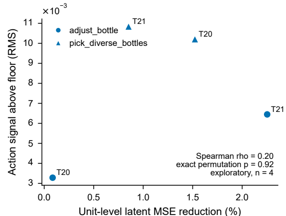
d State-action association is unresolved
