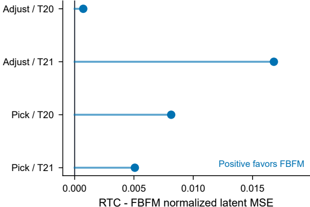
a All strict pairs favor FBFM
