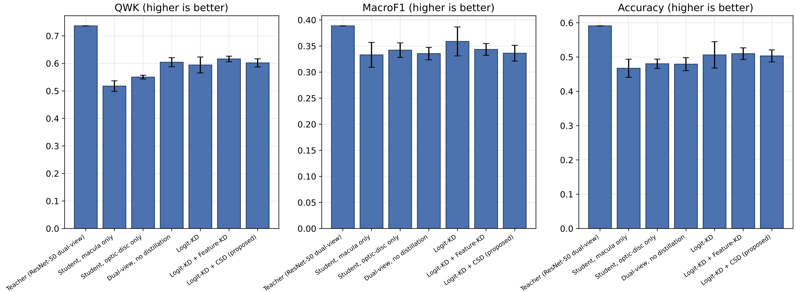
Figure 2 - Predictive performance on the DRTiD test set
