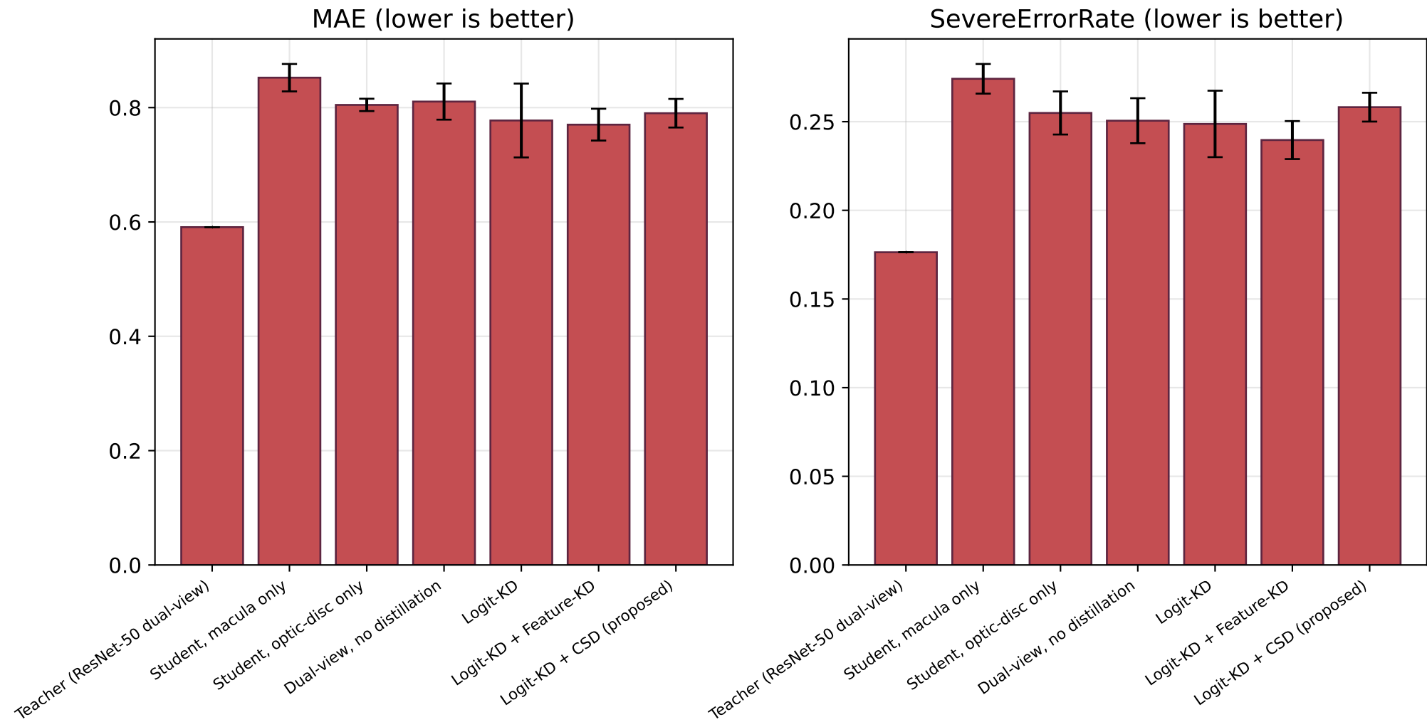
Figure 3 - Ordinal safety: MAE and severe-error rate
