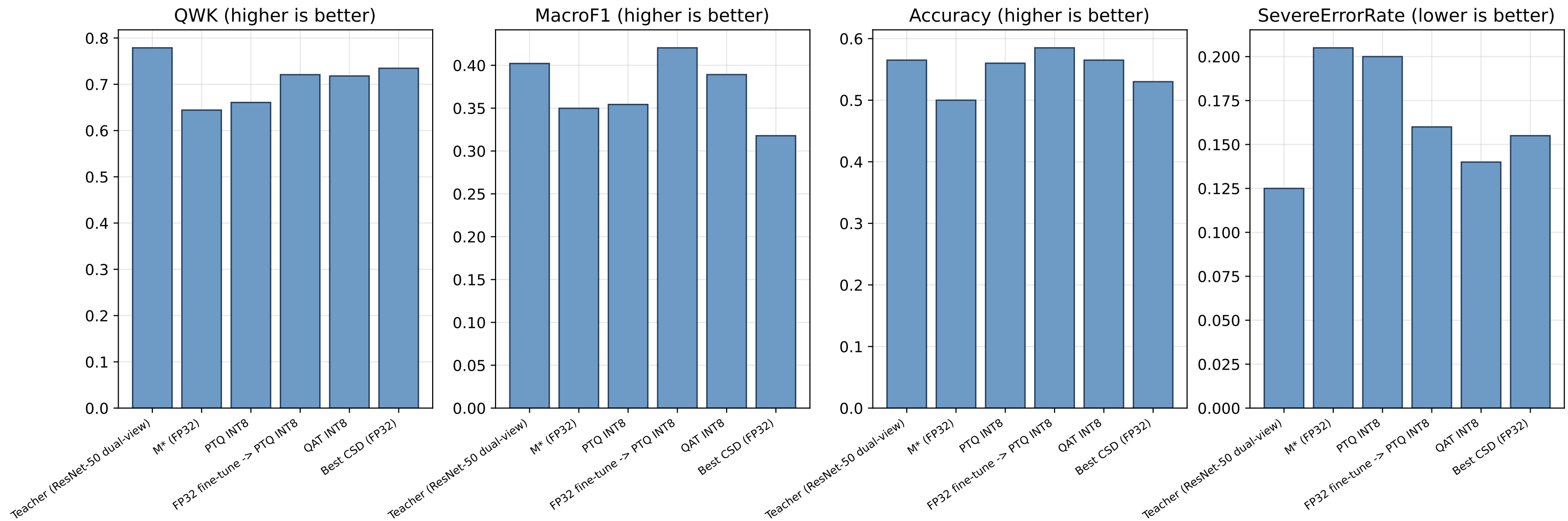
Figure 13 - DeepDRiD setC confirmatory external evaluation (_1=macula, frozen)
