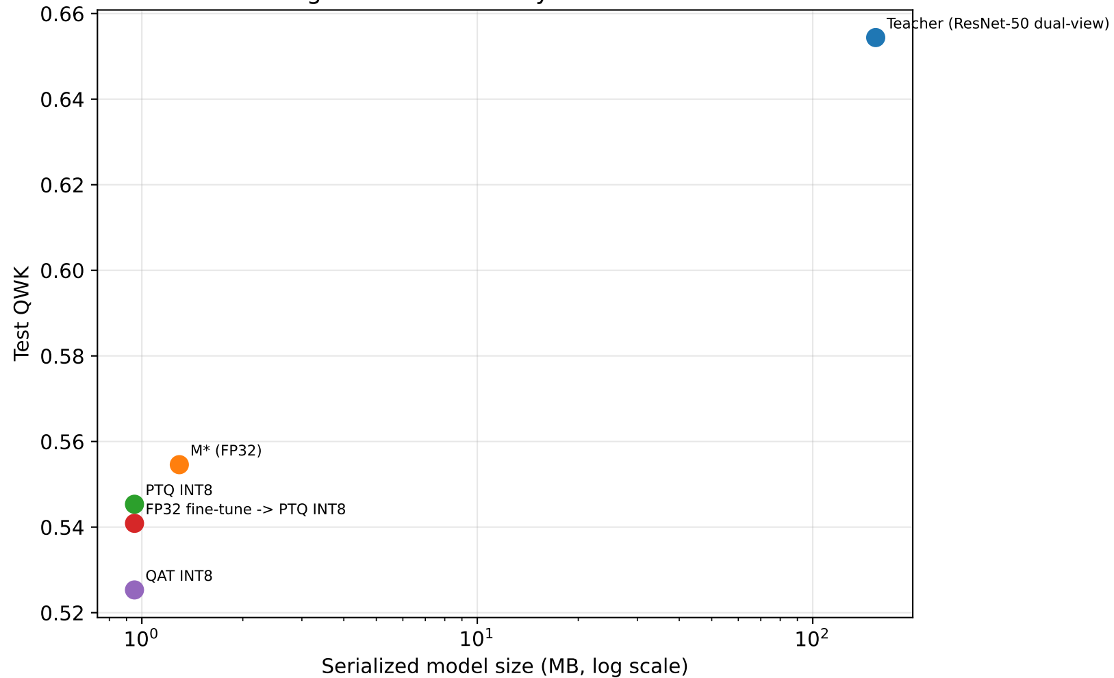
Figure 13 — Accuracy vs model size
