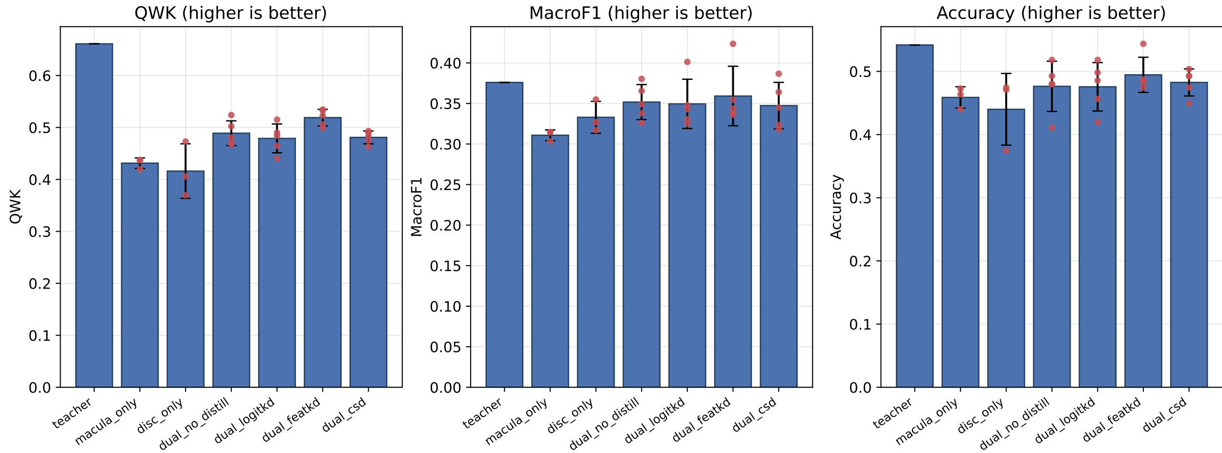
Figure 3 — Predictive performance on the internal DRTiD test set (mean \pm SD over seeds; dots = individual seeds)
