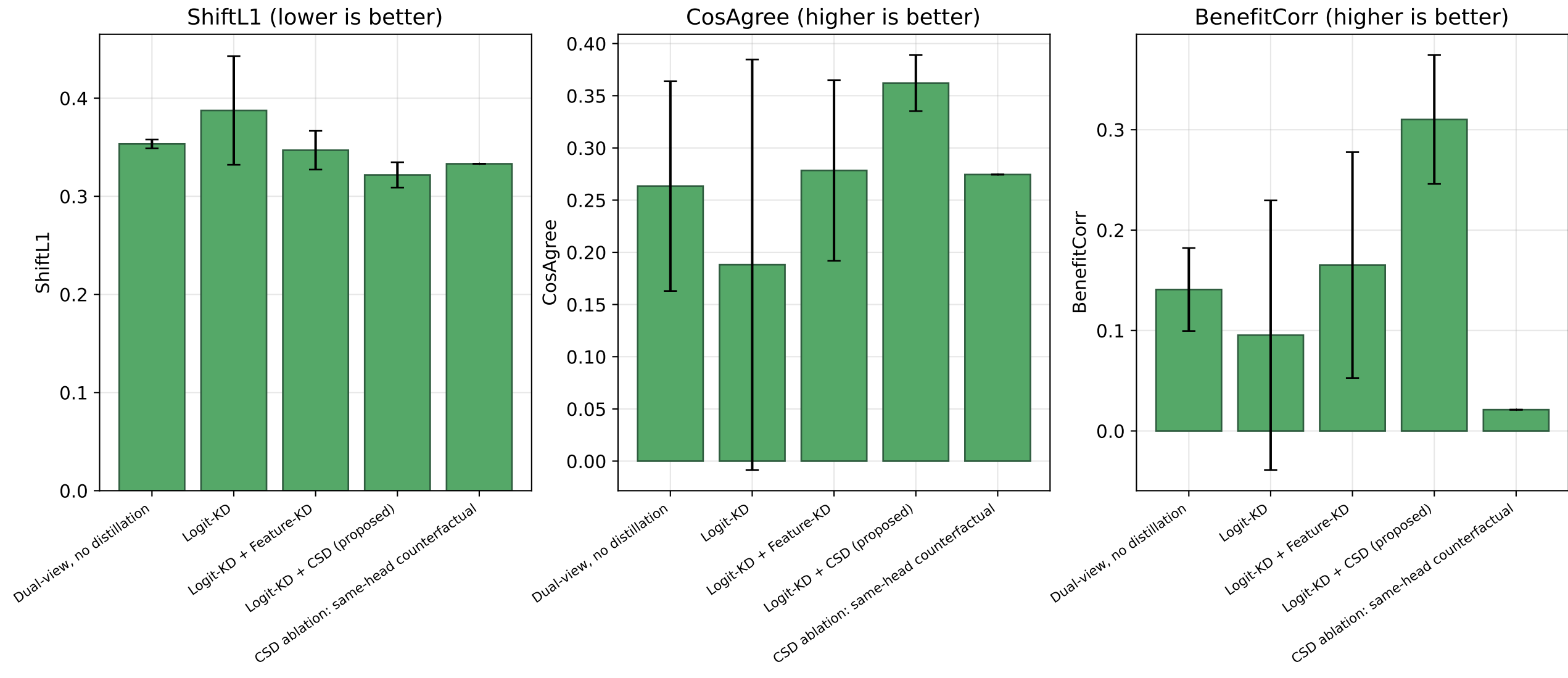
Figure 8 — CSD mechanism: is the teacher's complementarity shift actually transferred?
