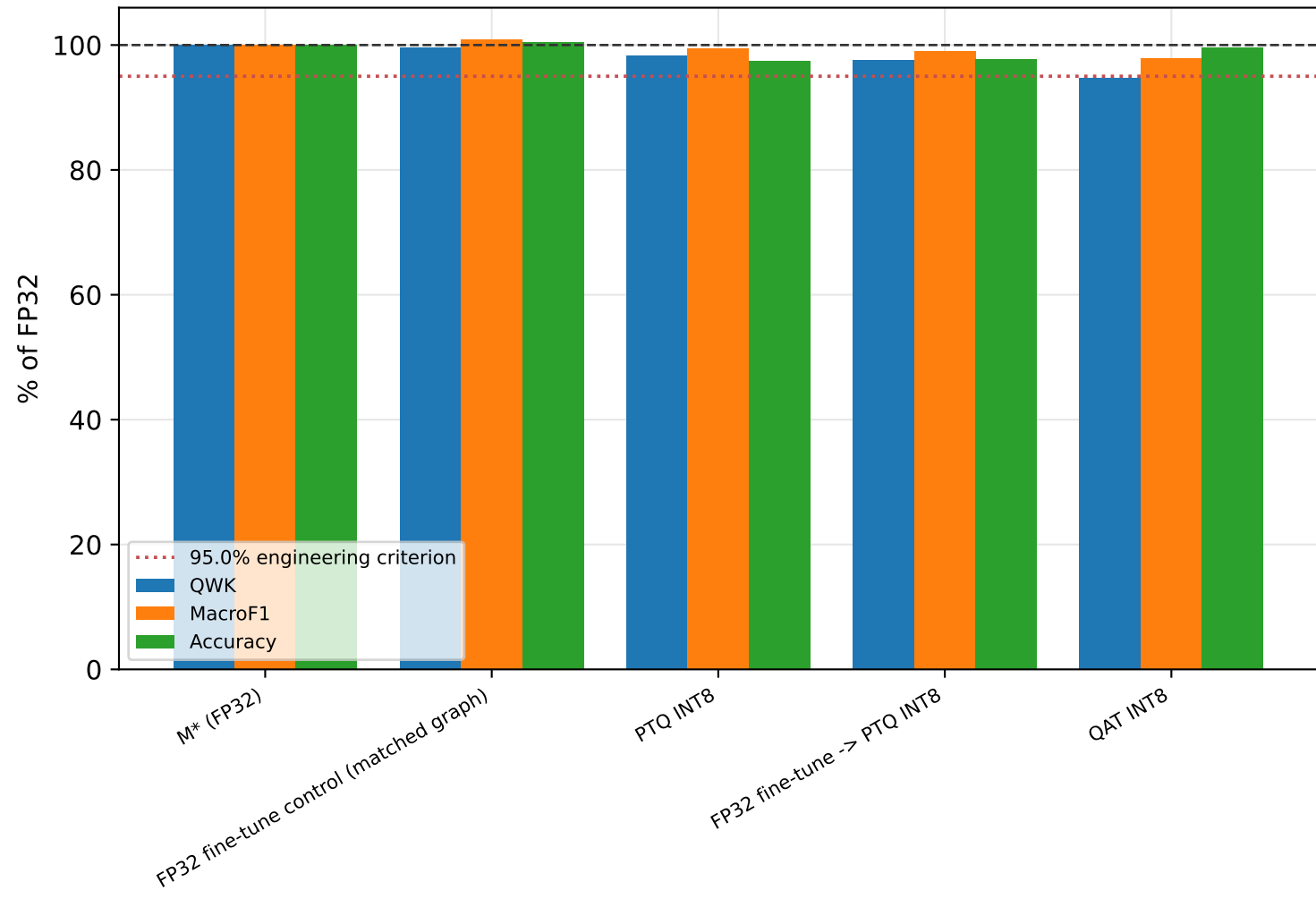
Figure 9 - Performance retention after quantization
