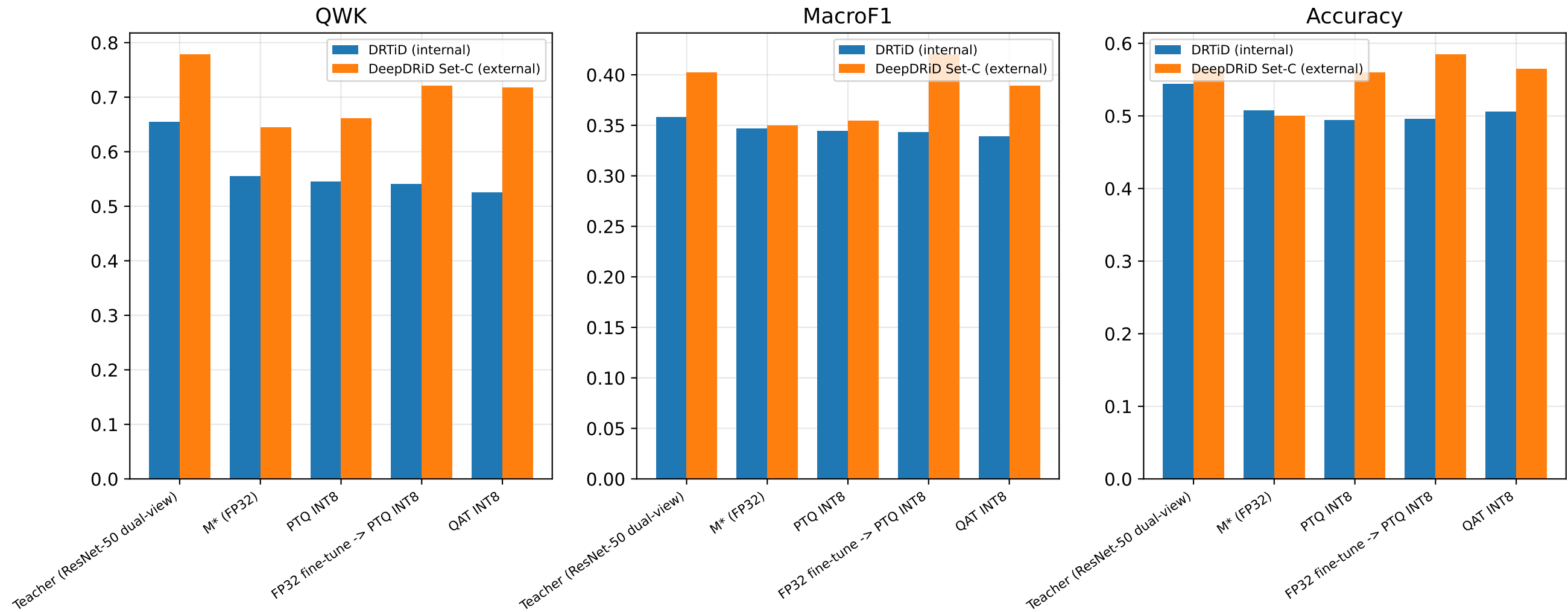
Figure 14 - Internal vs confirmatory external generalization
