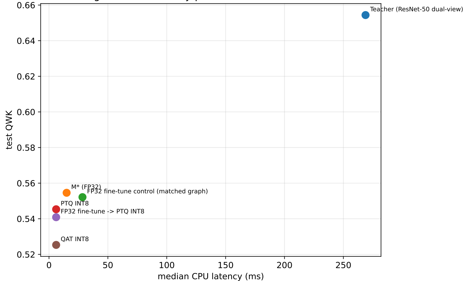
Figure 11 - Efficiency-performance Pareto frontier
