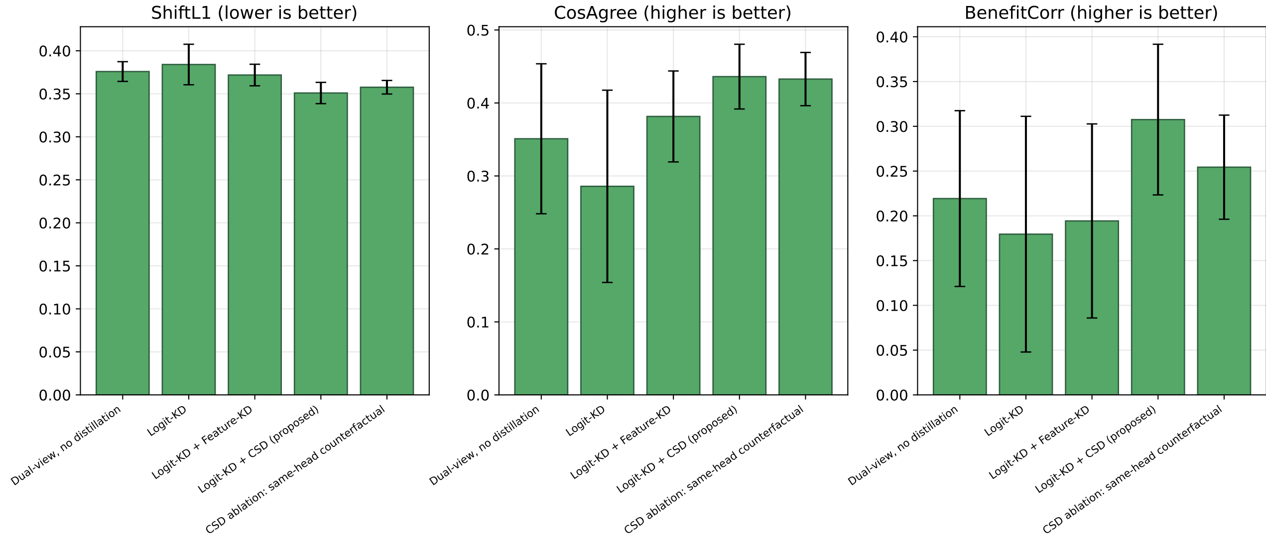
Figure 7 - CSD mechanism: was the teacher's decision shift transferred?
