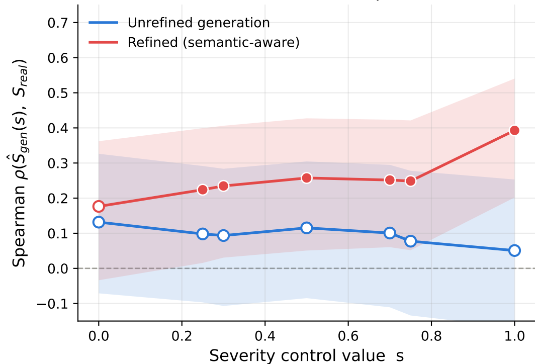
Probe: wildfire-finetuned \psi features
