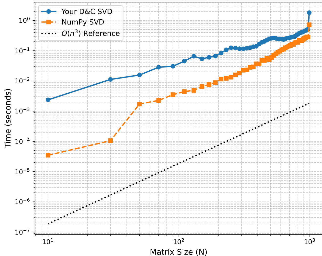
Runtime Complexity (Log-Log Scale)
