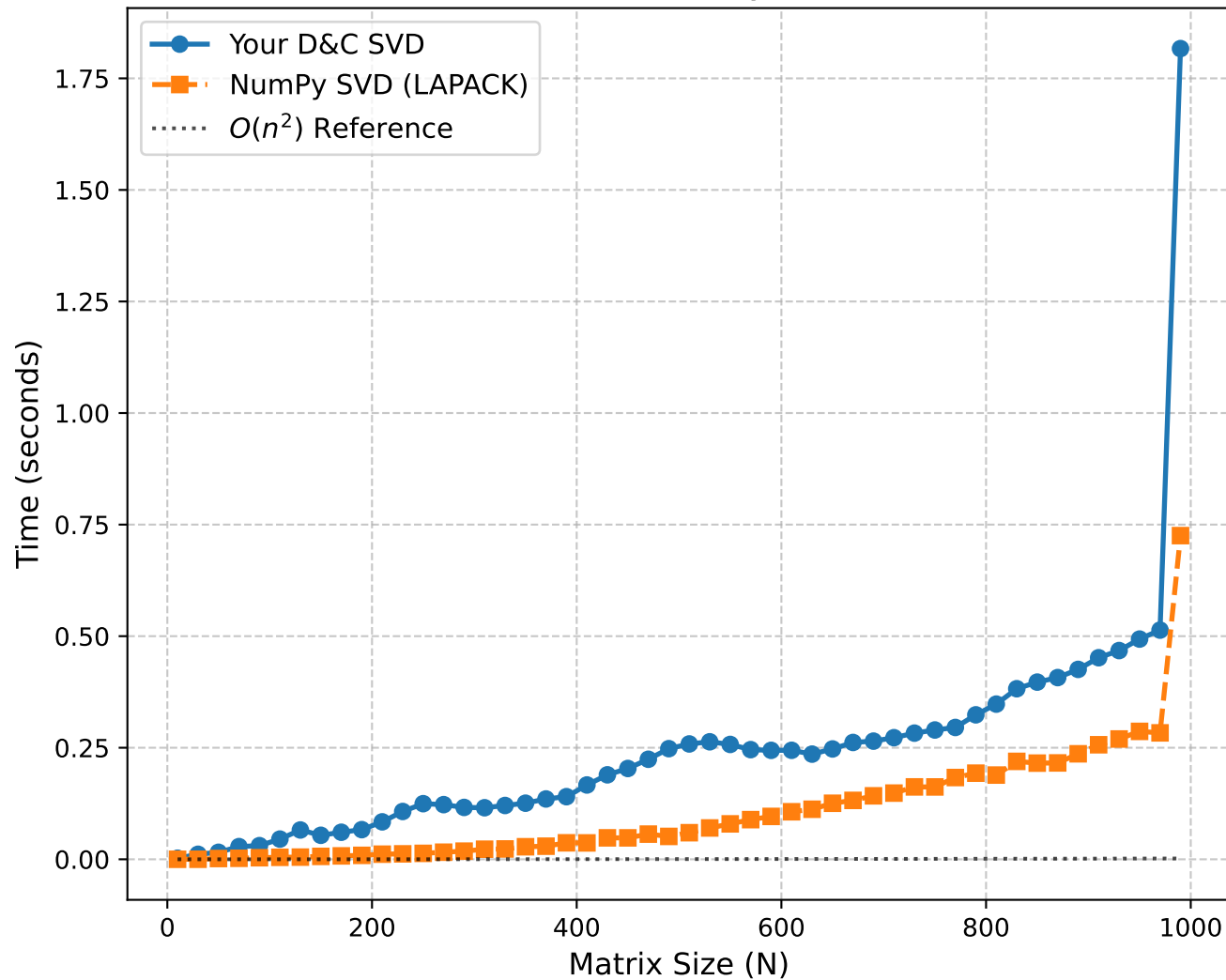
Runtime: D&amp;C vs NumPy (Linear Scale)
