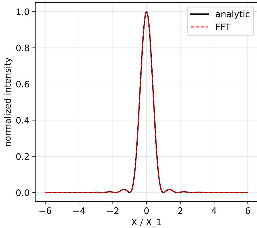
circle (Airy): central cut
