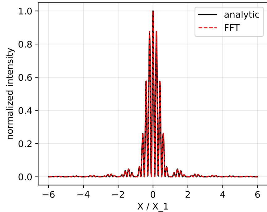
double slit (linear)
