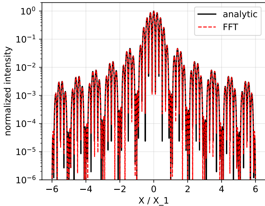
double slit (log)
