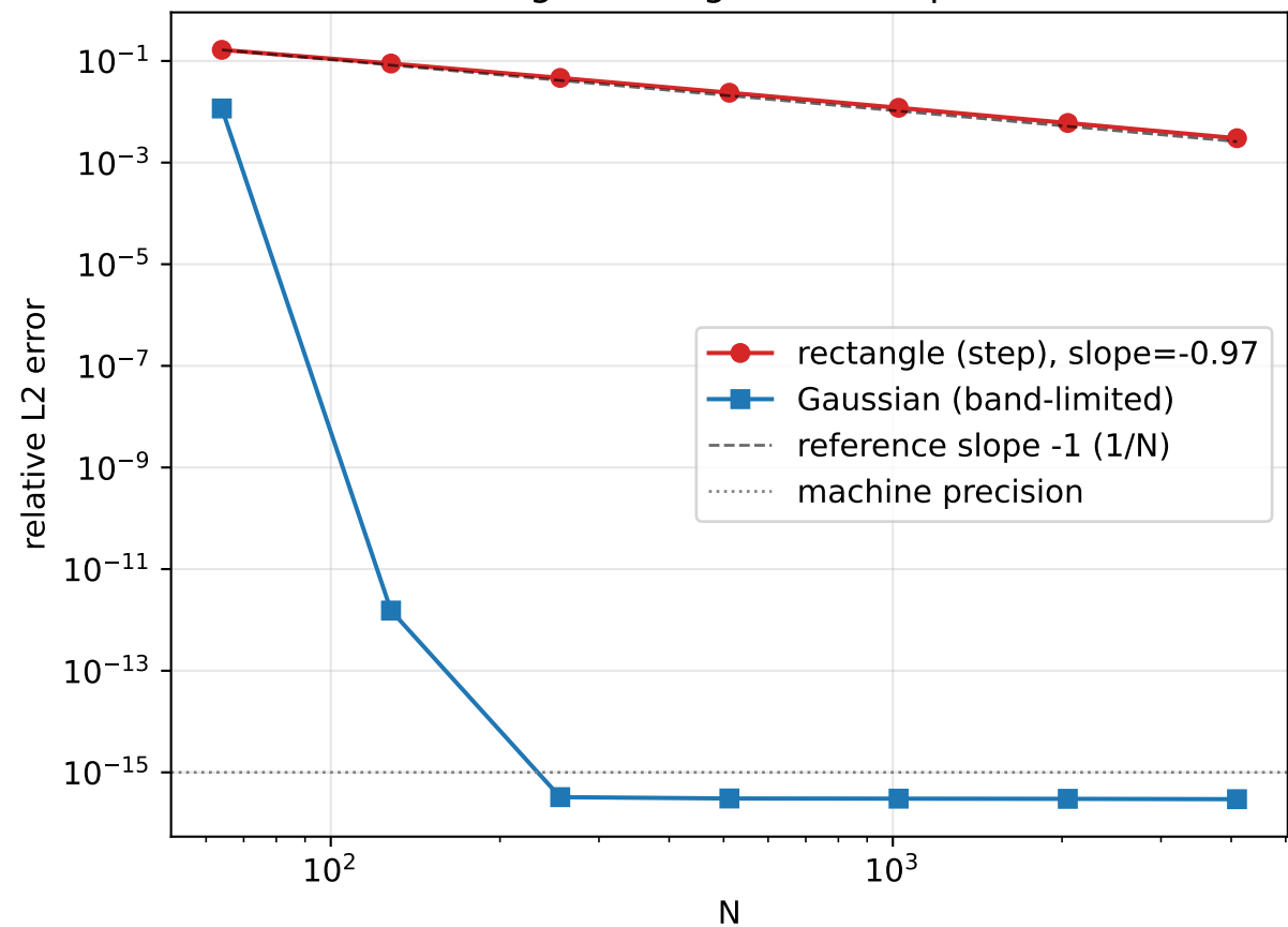
Convergence: algebraic vs spectral
