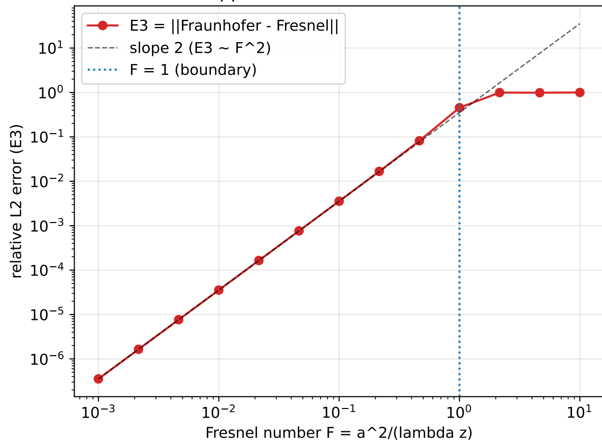
Fraunhofer approximation failure vs Fresnel number
