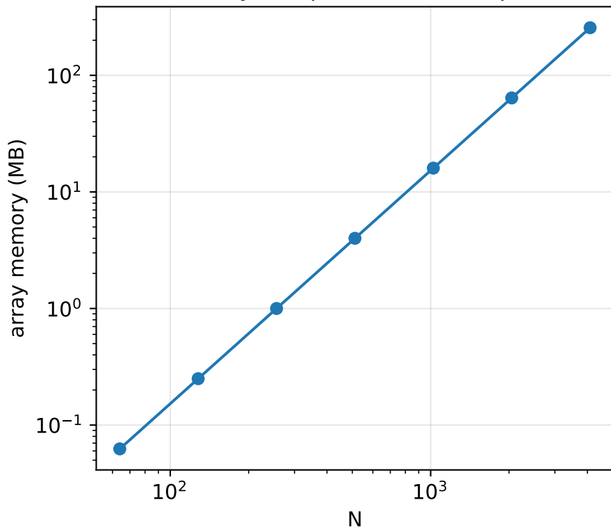
FFT memory footprint ( N^2 complex128)
