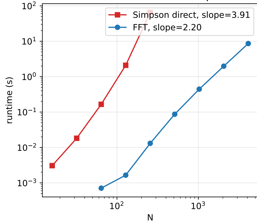
Runtime: FFT vs direct Simpson
