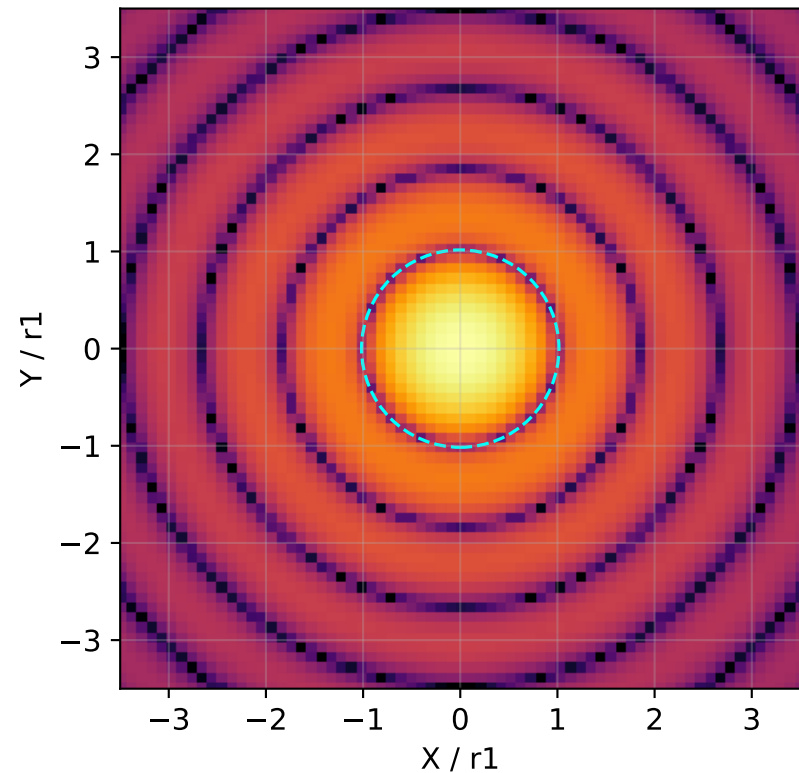
Airy pattern + recovered first ring
