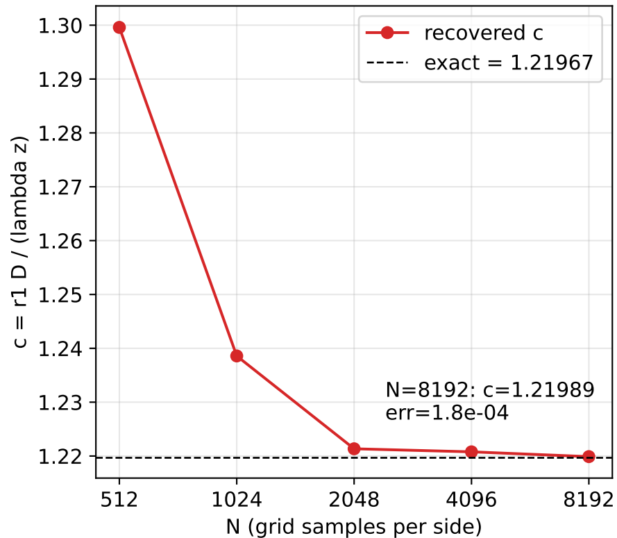
Convergence to the Rayleigh constant
