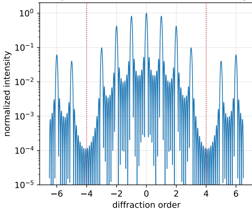
duty = 0.25: orders \pm 4 , \pm 8 ... missing
