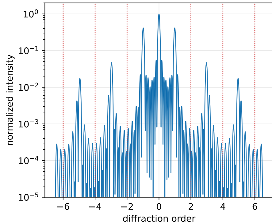
duty = 0.5: orders \pm 2 , \pm 4 ... missing
