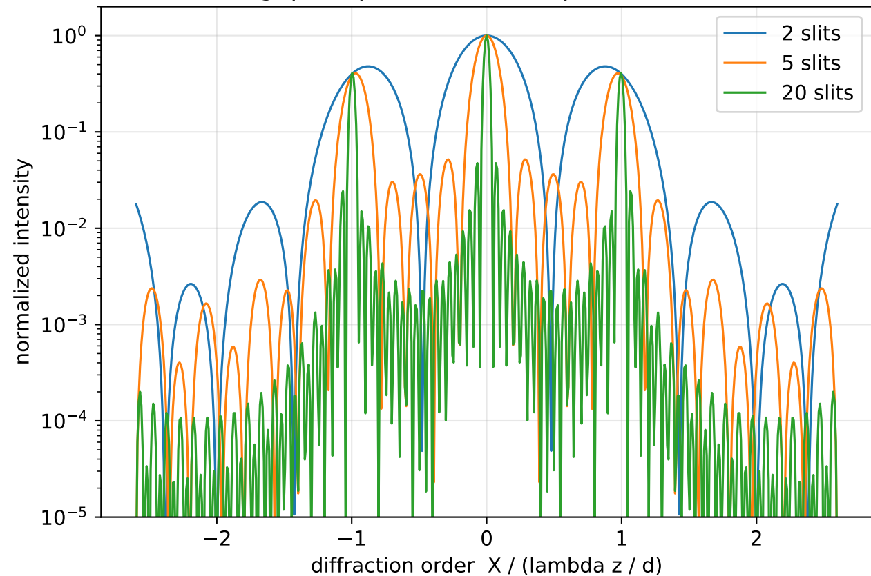
Grating: principal maxima sharpen with slit count
