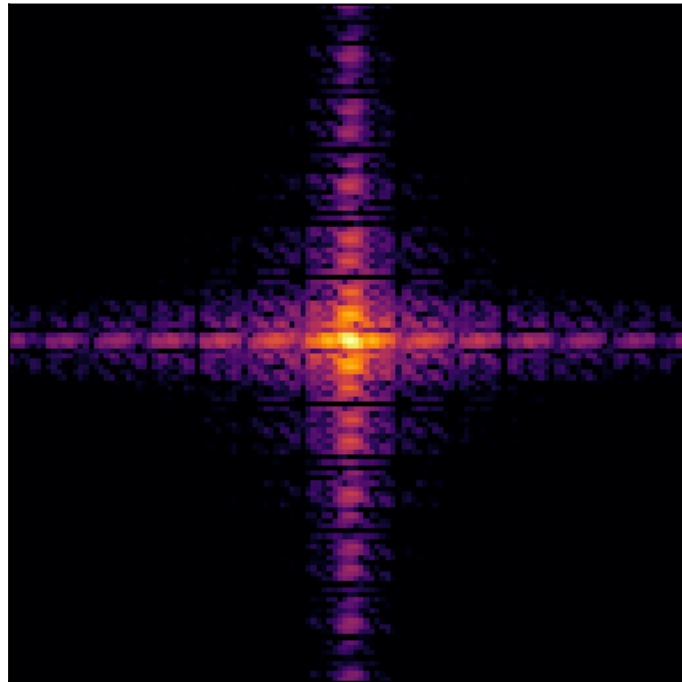
Fraunhofer pattern (log)
