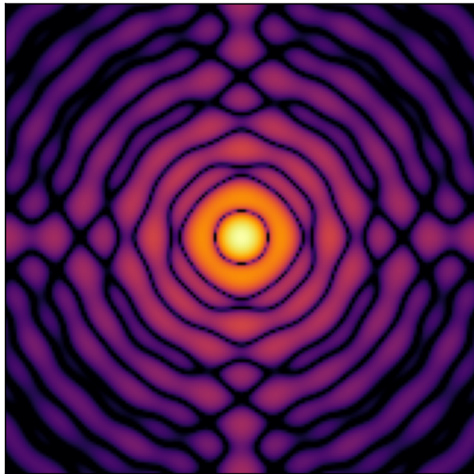
PSF (log): Airy core + diffraction spikes
