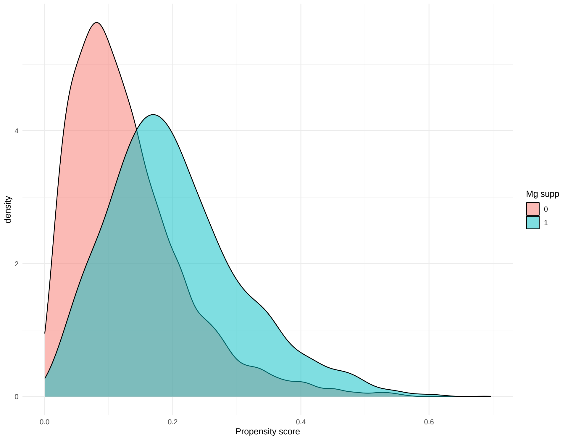
TTE-B (all patients): PS overlap
