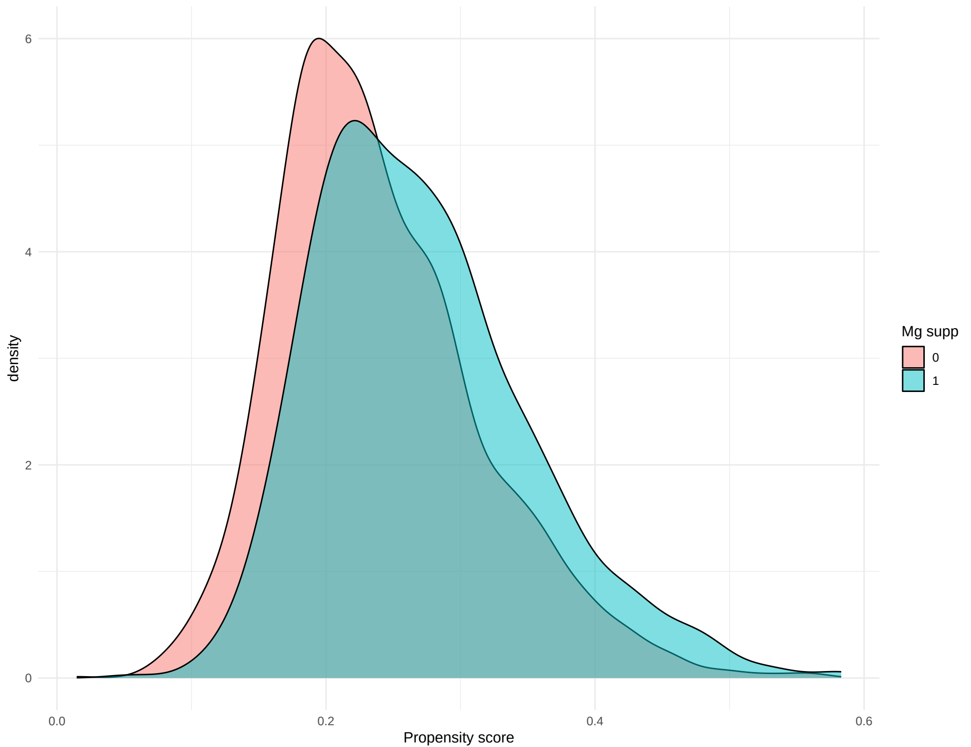
TTE-A (hypoMg): PS overlap
