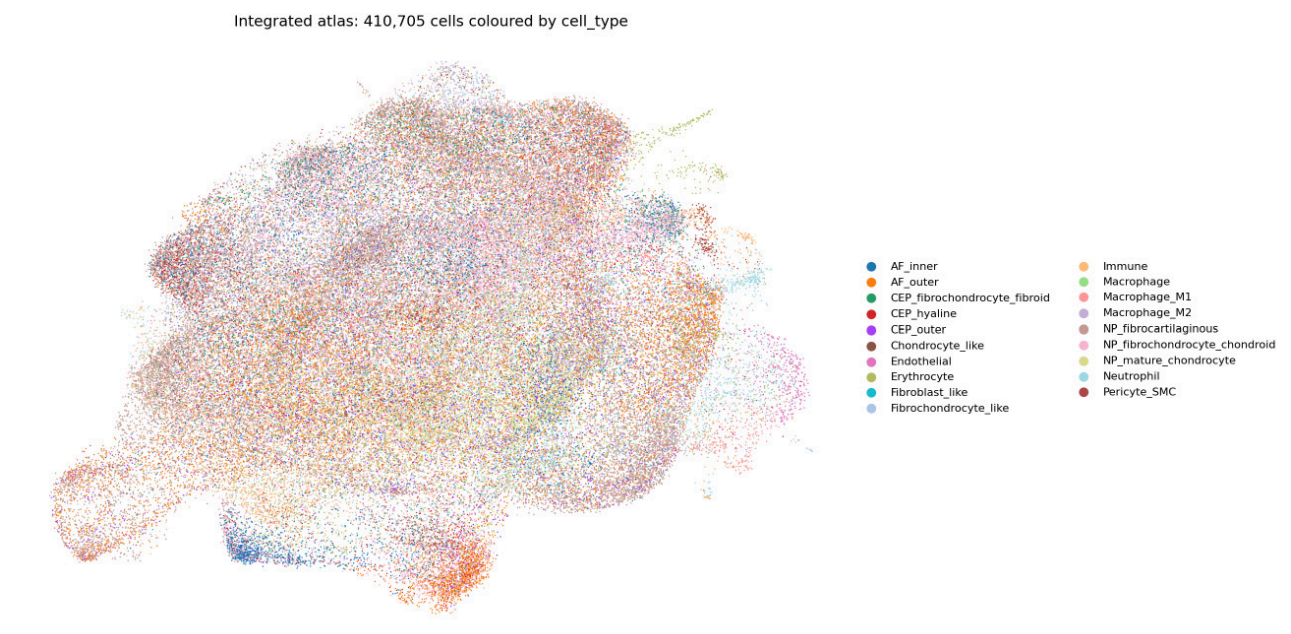
[Figure 1.] UMAP of the all-cells integrated atlas after tiered scVI integration and three-stage annotation. 410,705 cells coloured by cell_type . Mesenchymal populations (NP_fibrocartilaginous, NP_fibrochondrocyte_chondroid, NP_mature_chondrocyte, AF_inner, AF_outer, CEP_outer, CEP_hyaline, CEP_fibrochondrocyte_fibroid) and the non-mesenchymal lineages — vascular (Endothelial, Pericyte_SMC), immune (Macrophage_M1, Macrophage_M2, Neutrophil, Immune), and erythroid (Erythrocyte) — are clearly separated; within each compartment, related mesenchymal cell types are positioned as adjacent graded populations.
