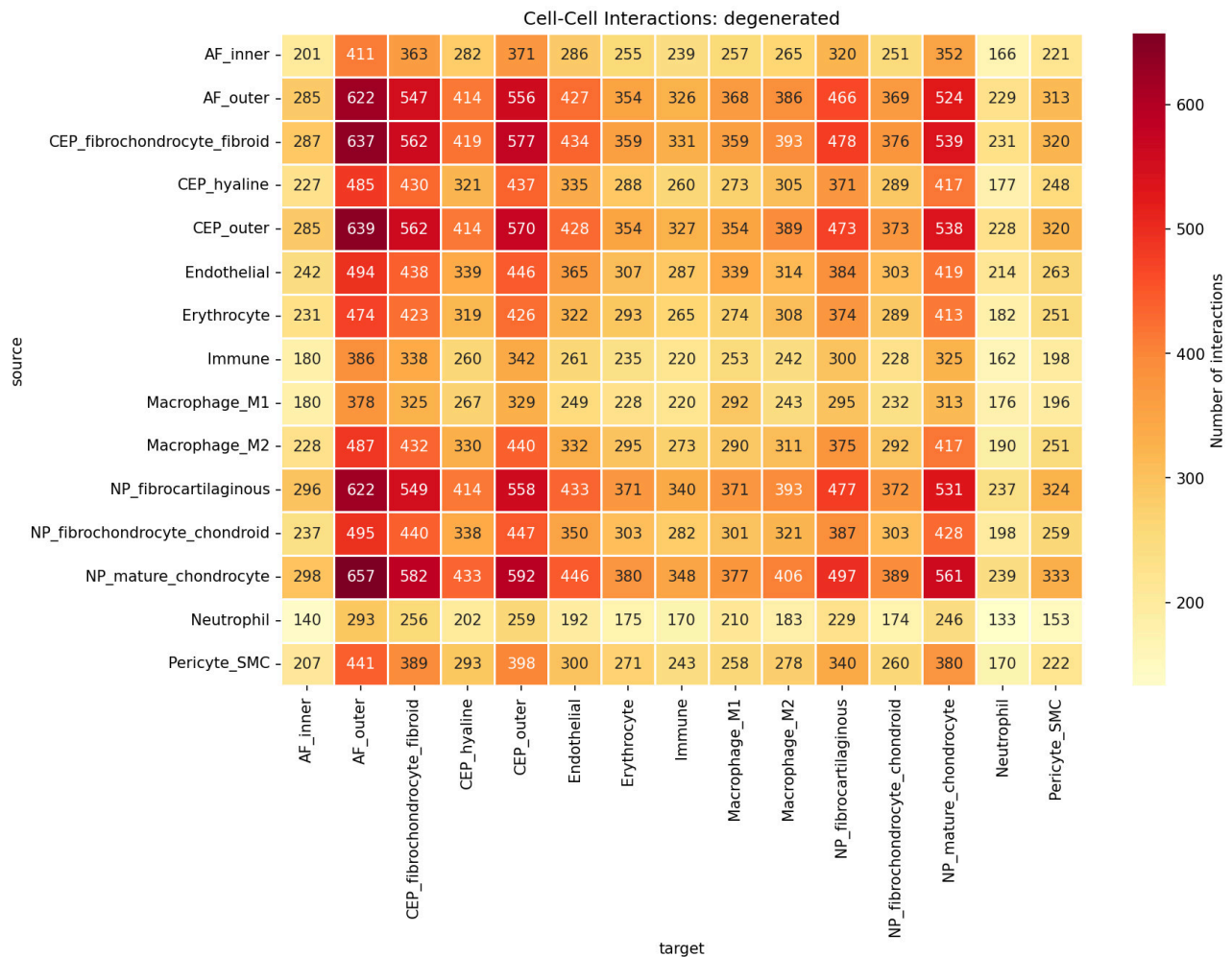
[Figure 9.] Cell-cell interaction heatmap in degenerated tissue. Source cell-type (rows) × target cell-type (columns) interaction counts. Mesenchymal cell types are heavily interconnected; non-mesenchymal populations show more focused interaction profiles.
