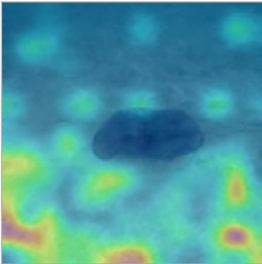
Grad-CAM overlay
