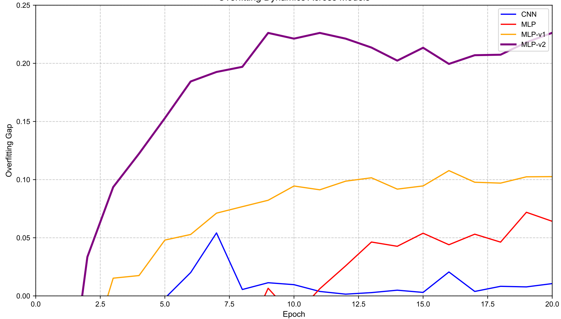
Overfitting Dynamics Across Models
