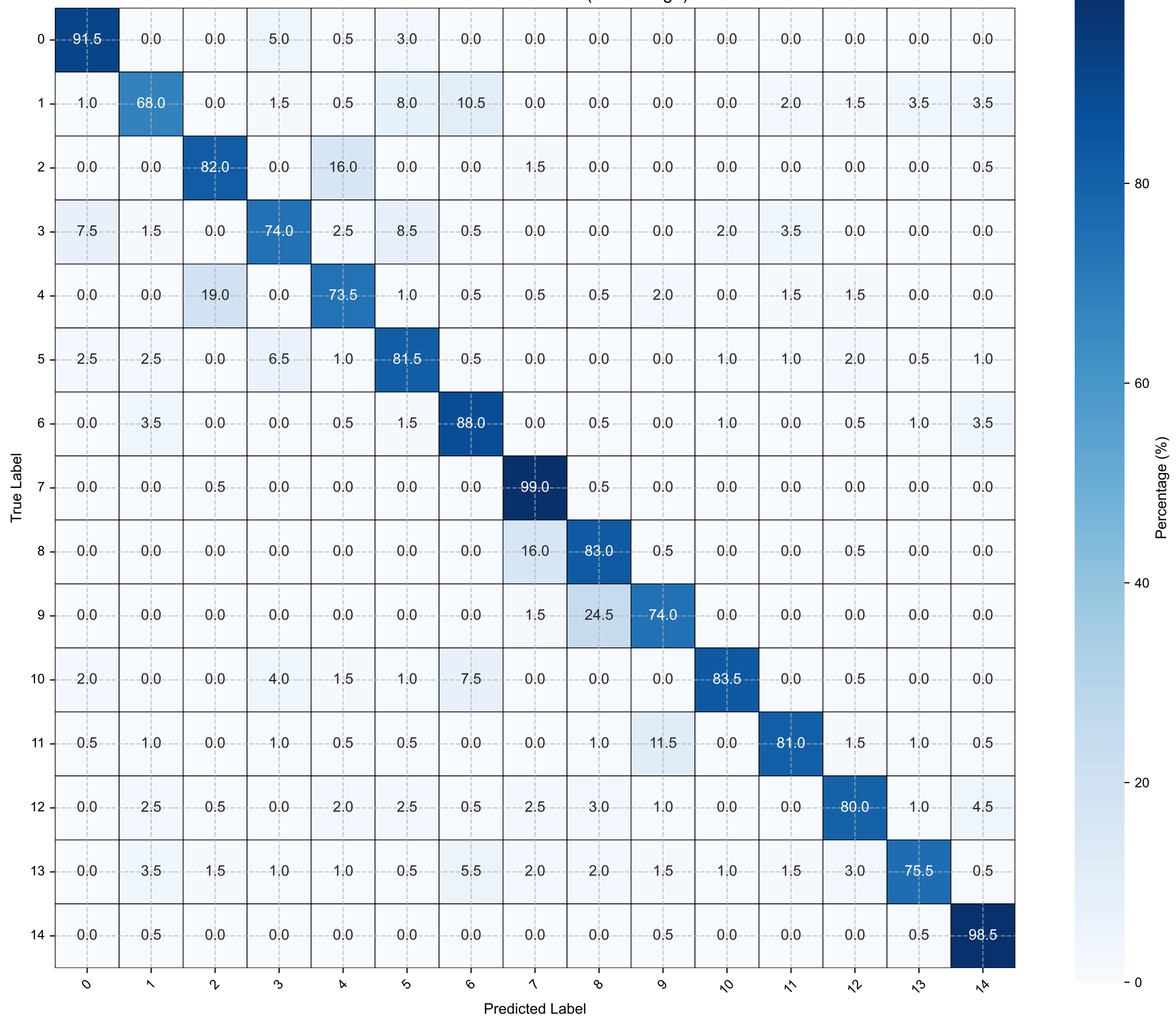
Confusion Matrix for MLP (Percentage)
