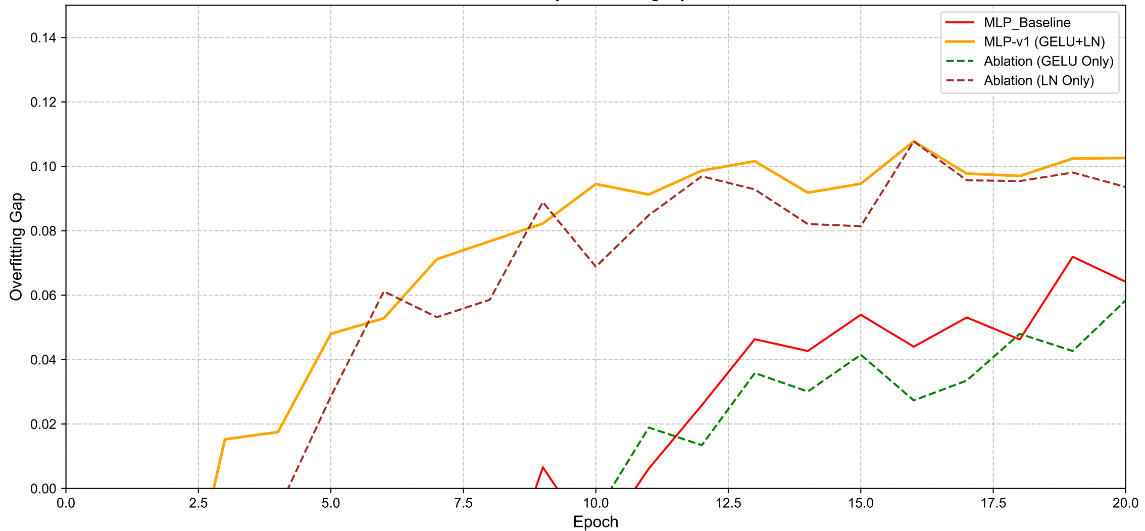
Ablation Study: Overfitting Dynamics
