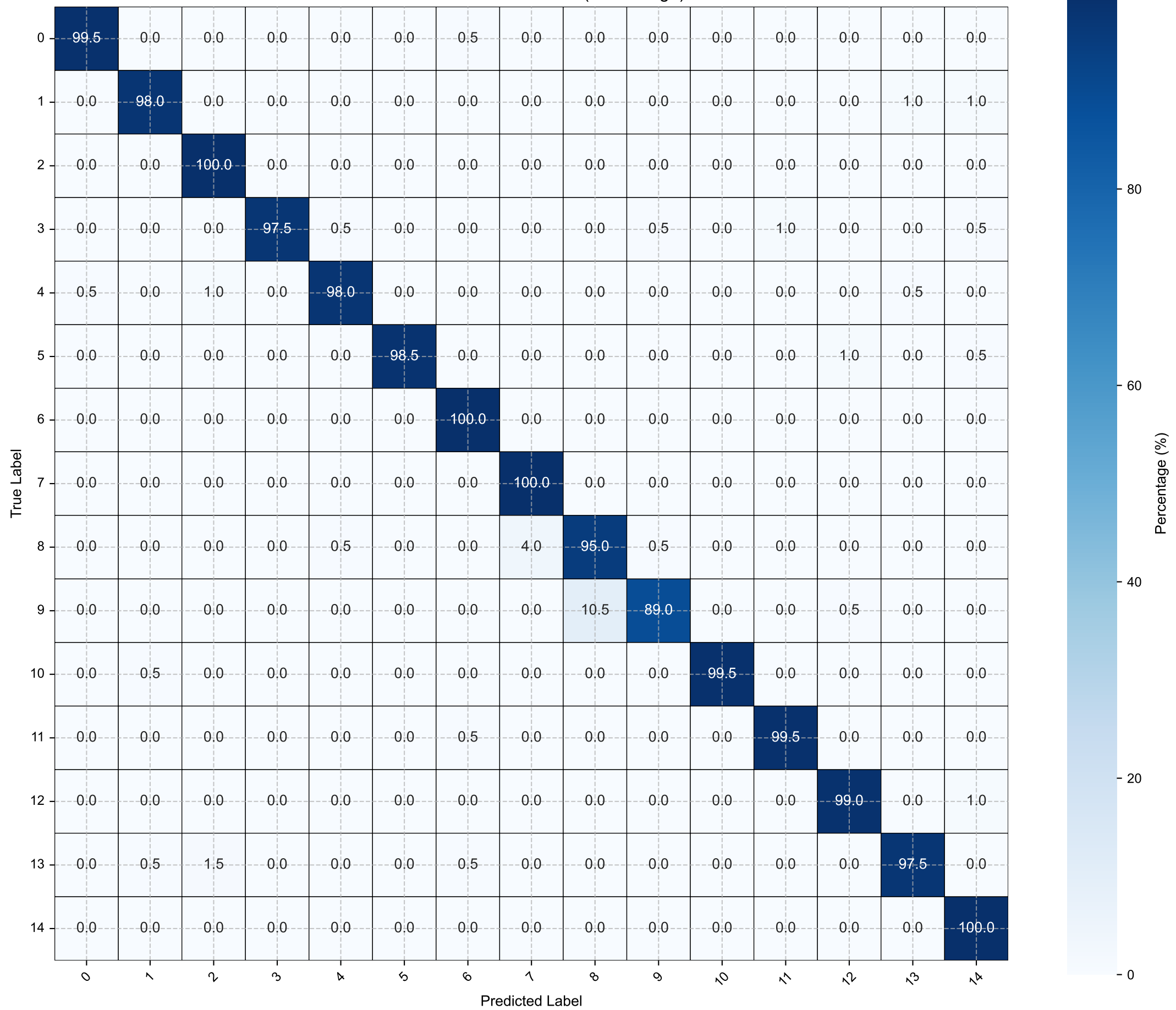
Confusion Matrix for CNN (Percentage)
