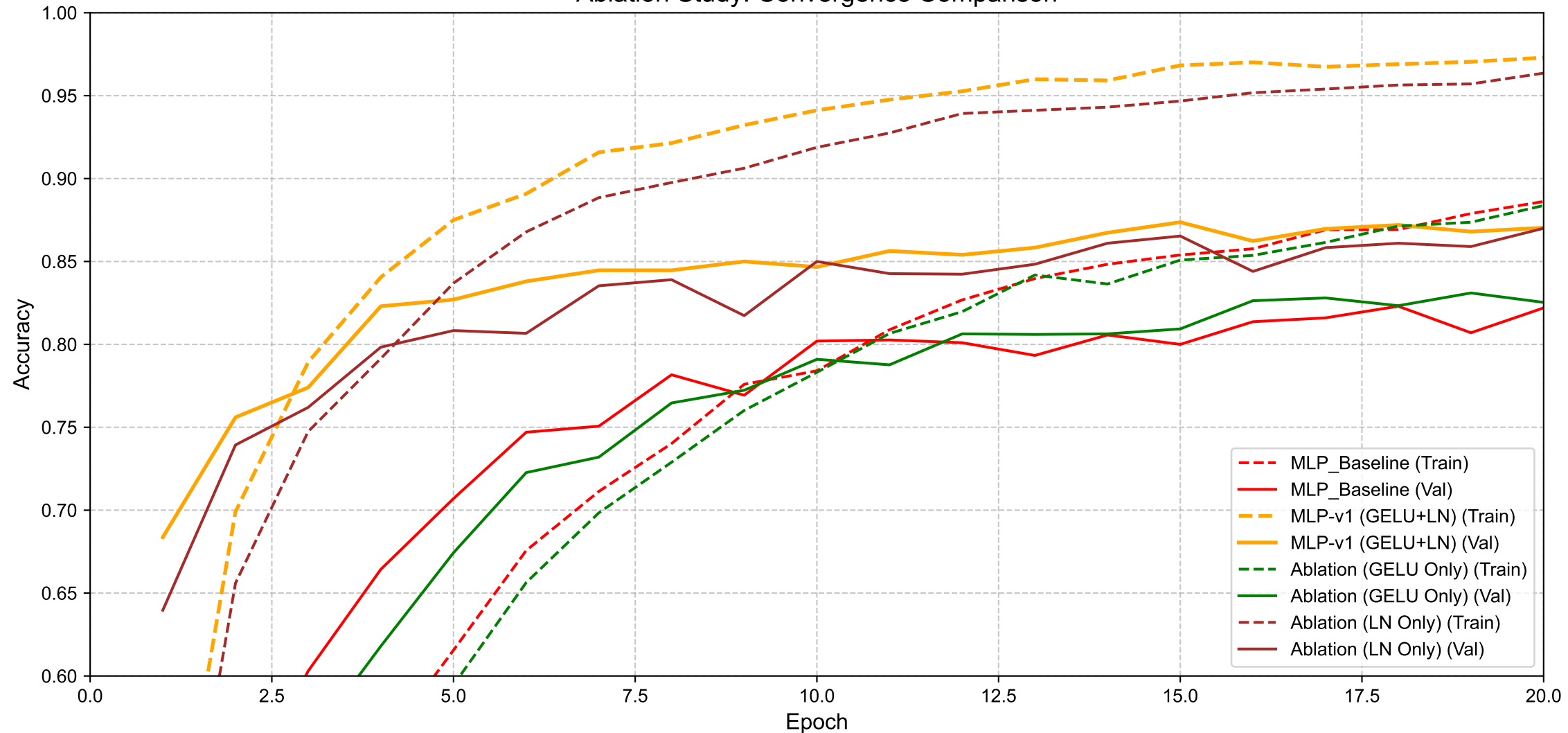
Ablation Study: Convergence Comparison
