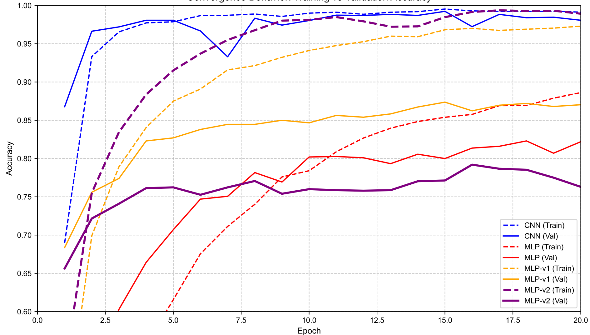
Convergence Behavior: Training vs Validation Accuracy
