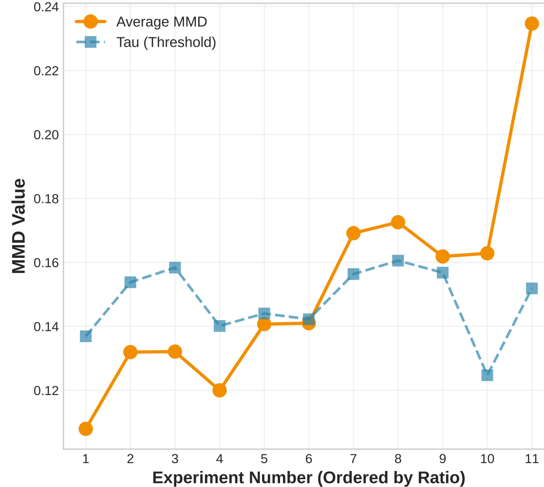
Average MMD vs Sample Ratio
