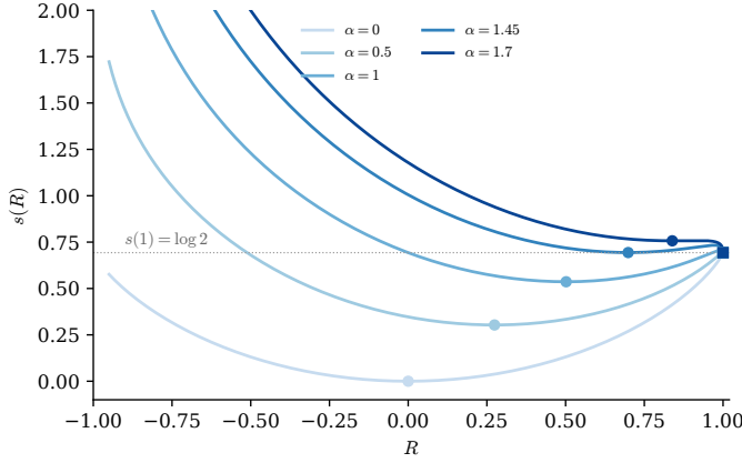
Figure 15: The annealed action s(R) of the Ising perceptron, (2.44), for several loads. Interior local minima are marked with circles; the teacher state R = 1 , where s(1) = \log 2 exactly, with squares. The two basins exchange dominance near \alpha \approx 1.45 .
