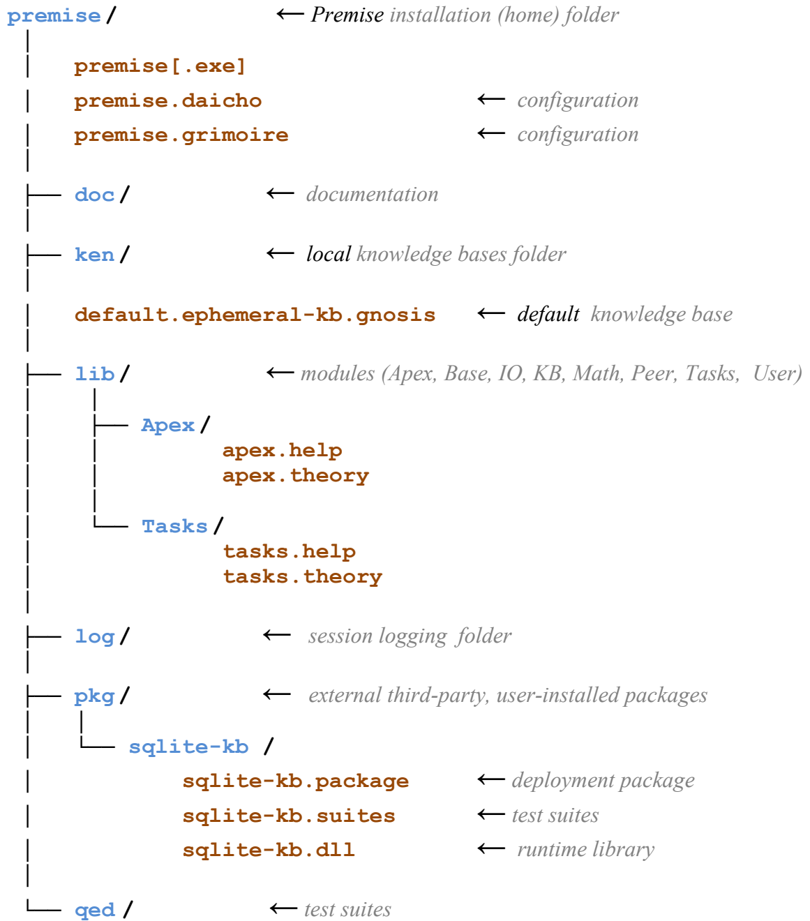
Figure 1. Premise folder hierarchy
