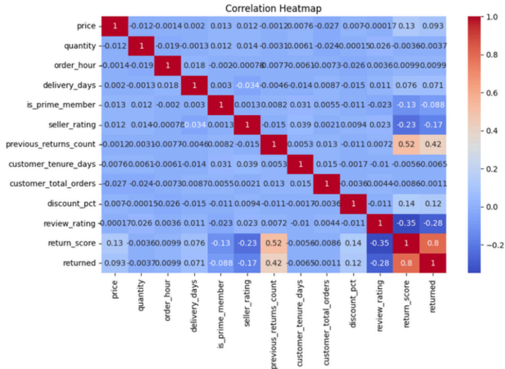
Figure 6: Correlation Heatmap
