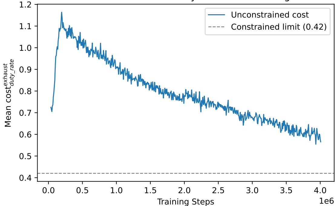
Unconstrained Exhaust Duty-Rate Cost Convergence
