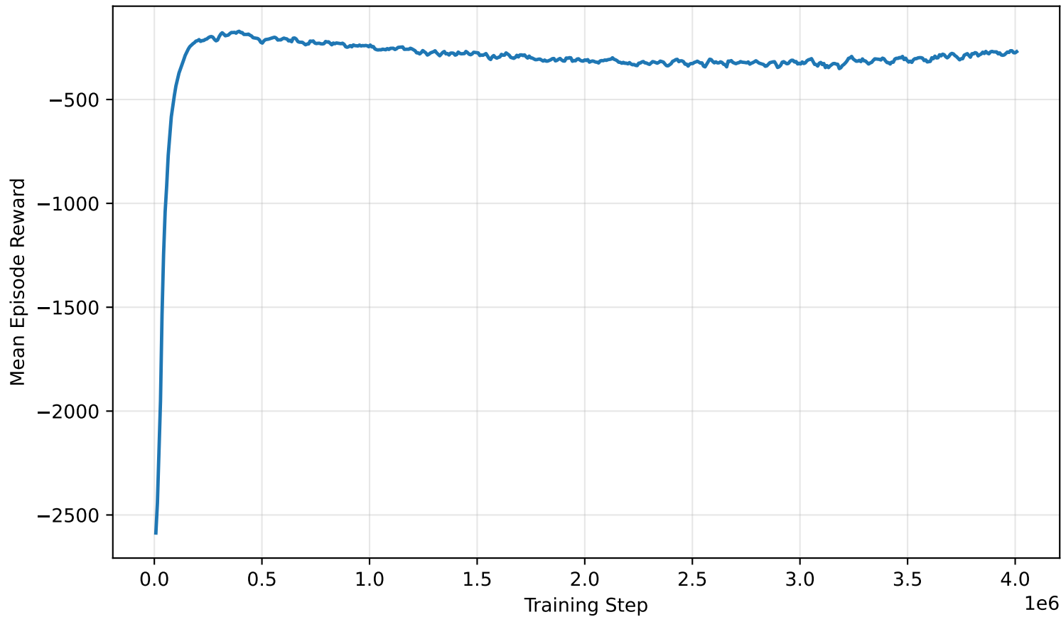
Mean Episode Reward During Training
