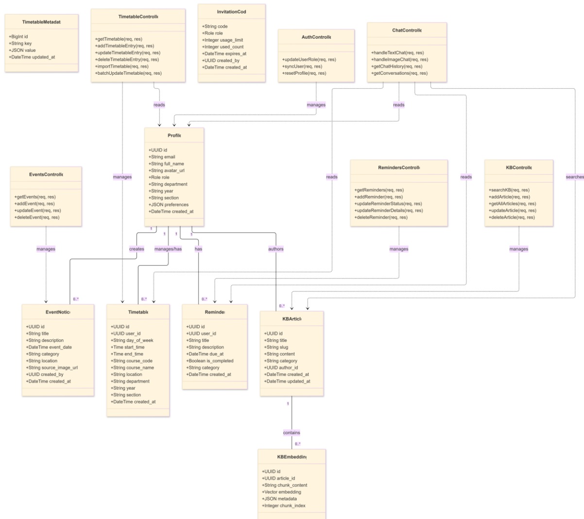
Fig.5.1.2 Class diagram
