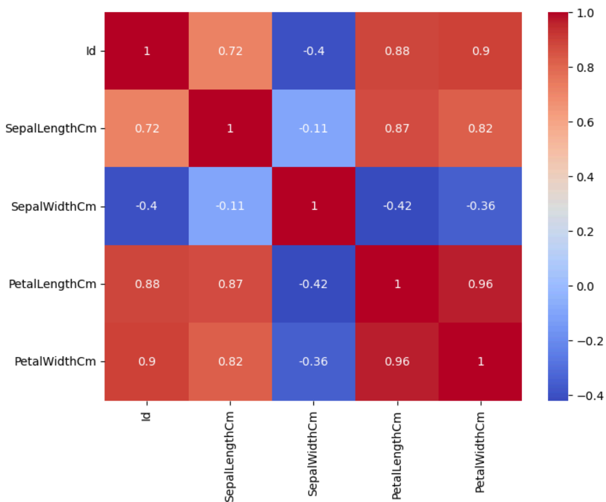
Correlation Heatmap
