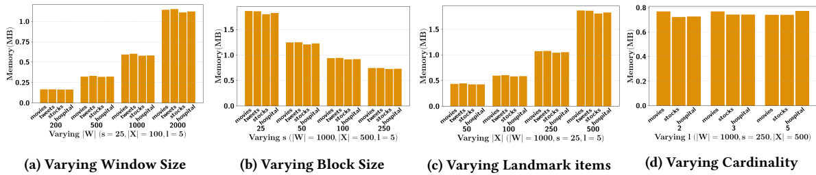
Figure 13: Query Processing with BFair-ReOrder Memory Consumption over 5000 windows
