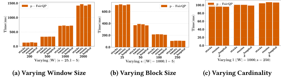
Figure 12: Total Query processing running time without BFair-ReOrder for 5000 read-only windows
