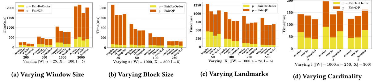
Figure 11: Total Query processing running time with BFair-ReOrder for 5000 windows
