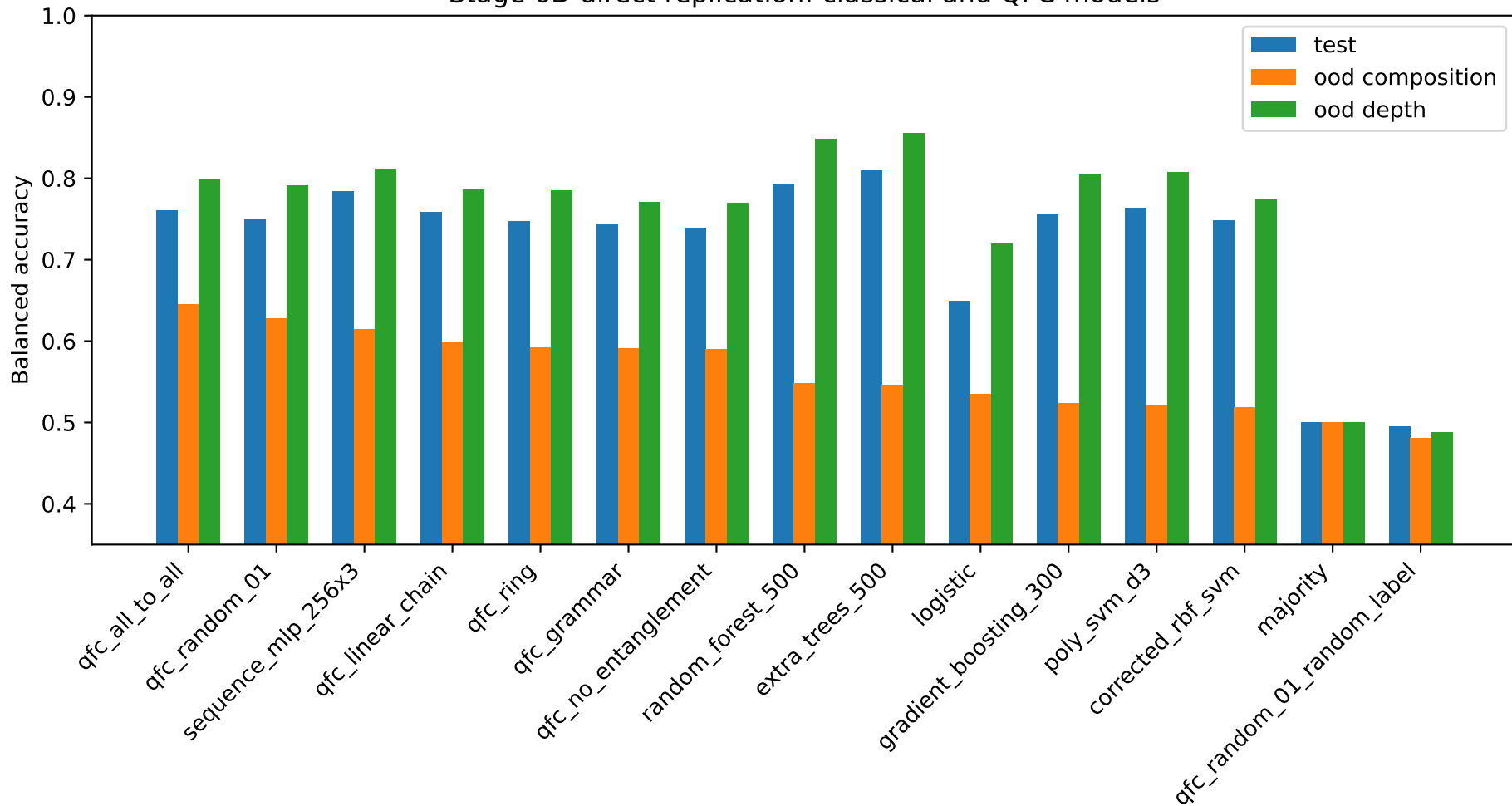
Stage 6D direct replication: classical and QFC models
