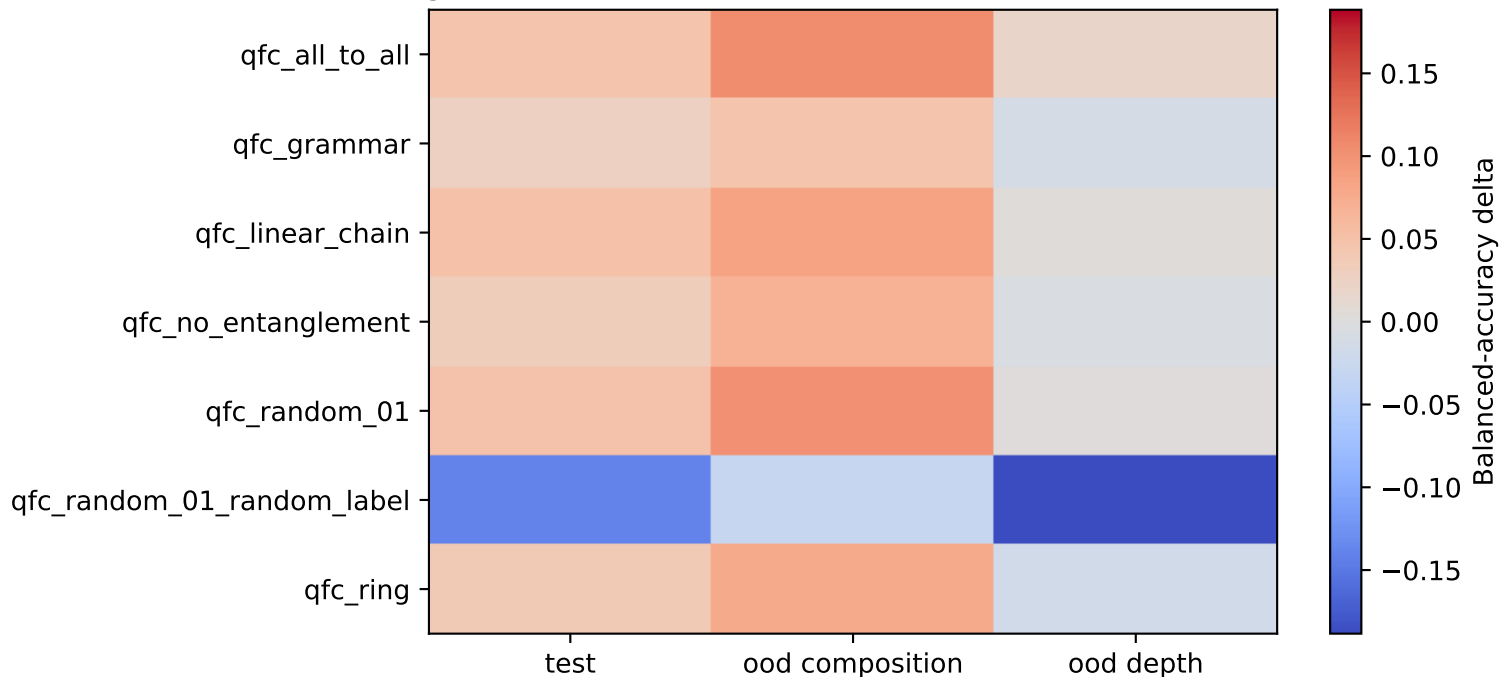
Stage 6D trained QFC kernel minus selected classical kernel
