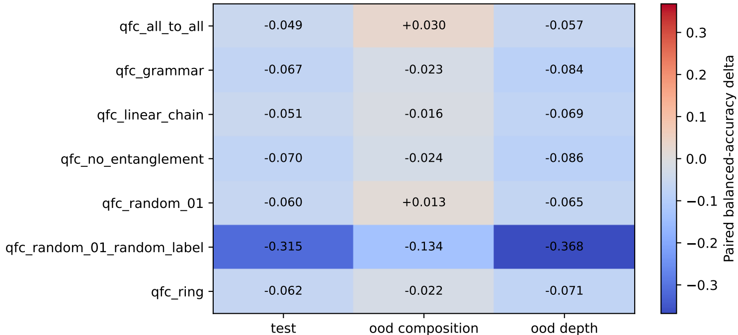
Stage 6D QFC delta versus pre-registered best classical comparator
