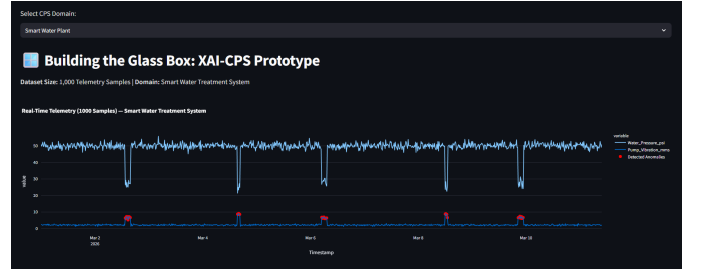
Fig. 1. The Streamlit “Glass Box” interface visualizing the synthesized 1,000-sample telemetry stream, with algorithmically detected anomalies highlighted in red.
