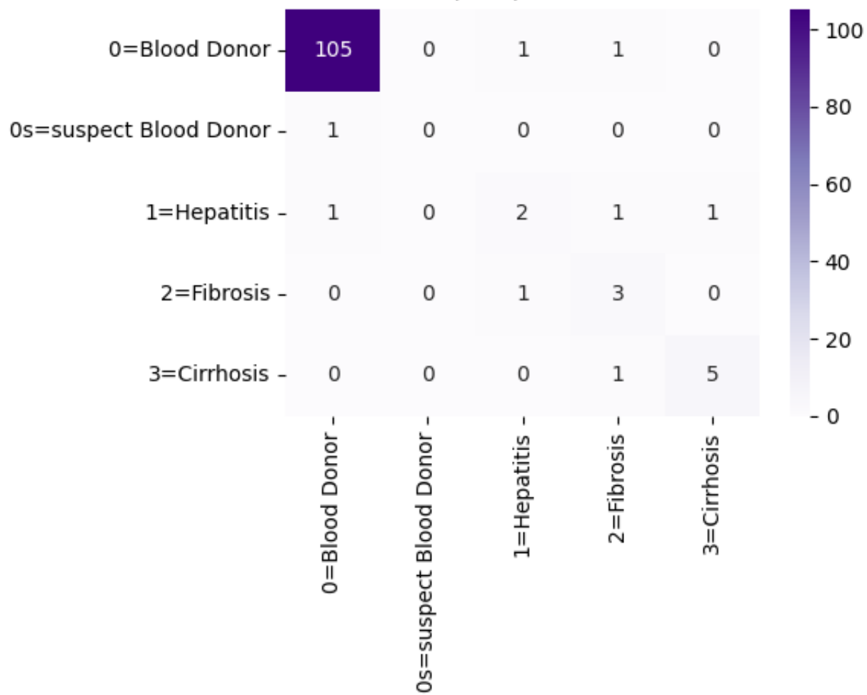
Final Model (MLP) Confusion Matrix
