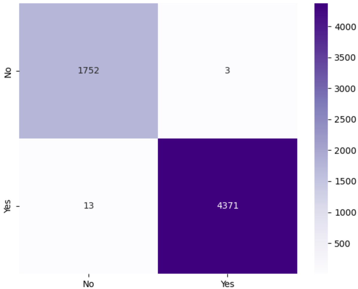
Final Model (RandomForest) Confusion Matrix
