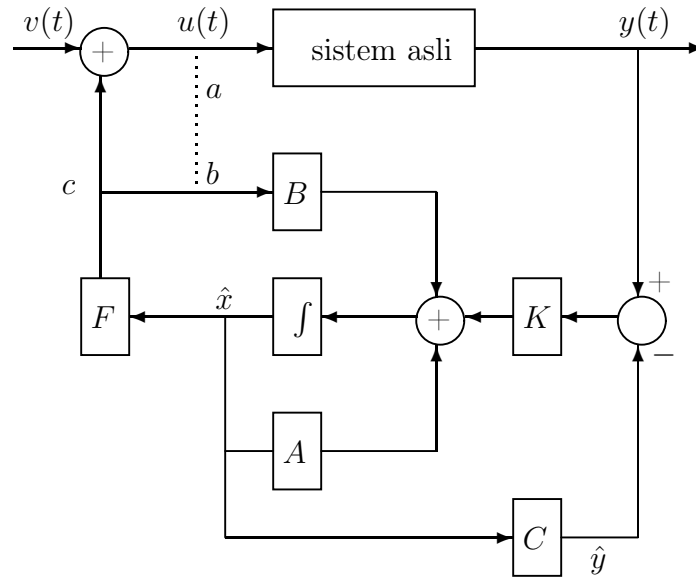
Gambar 5.5: Peyederhanaan diagram.
