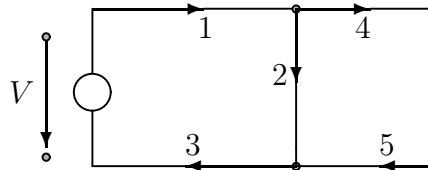
Gambar 2.1: Hukum Kirchhoff.
