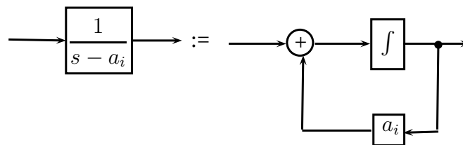
Gambar 7.9: Diagram Blok realisasi \frac{1}{s - a_i}
