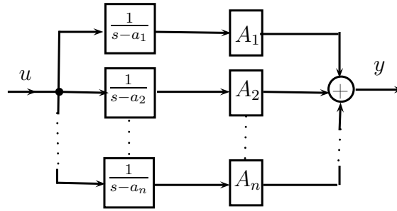
Gambar 7.8: Realisasi diagonal.
