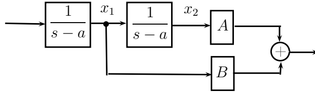
Gambar 7.10: Diagram Blok h(s)
