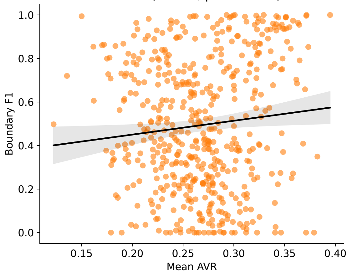
Mamba ( r=0.10 , p=2.29e-02 )
