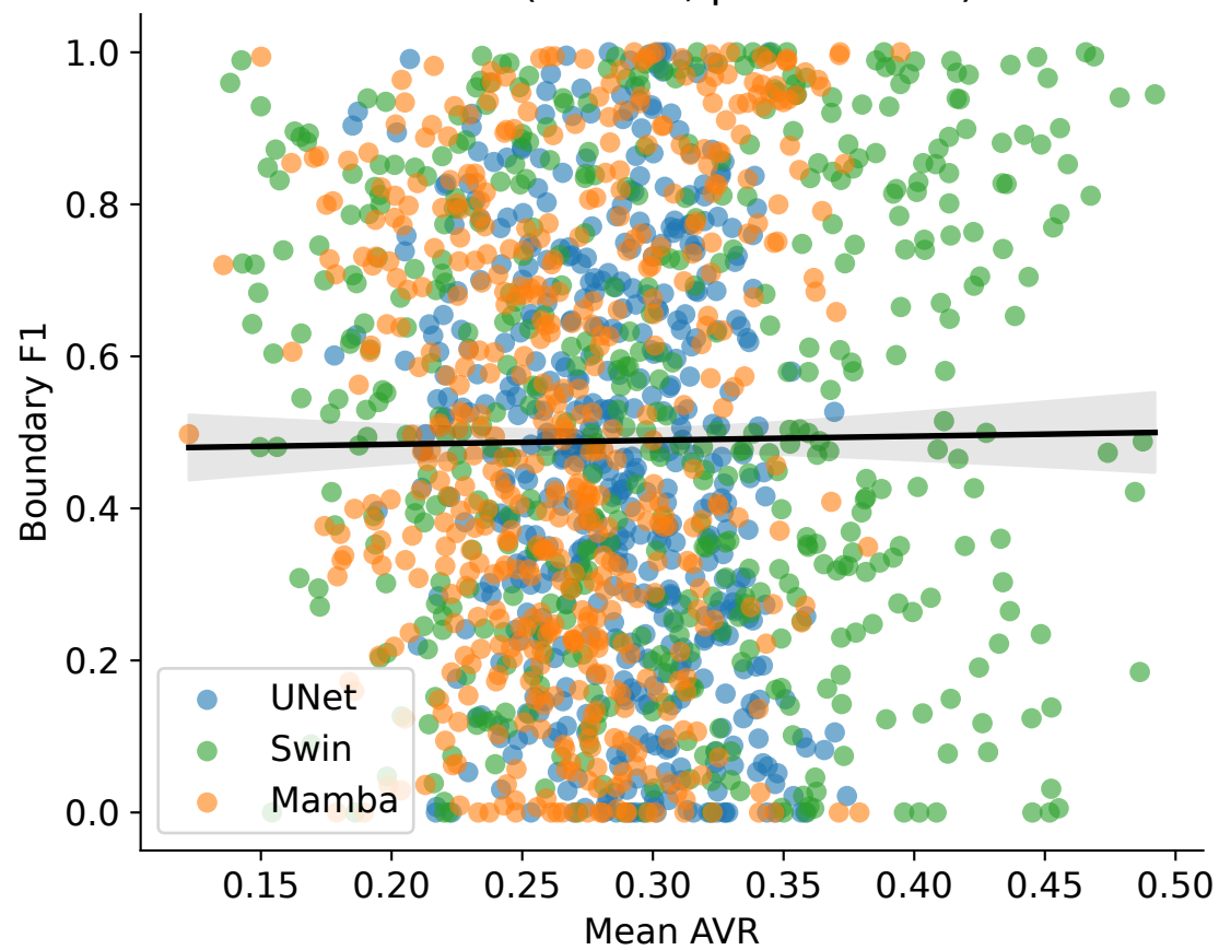
Pooled ( r=0.01 , p=6.70e-01 )
