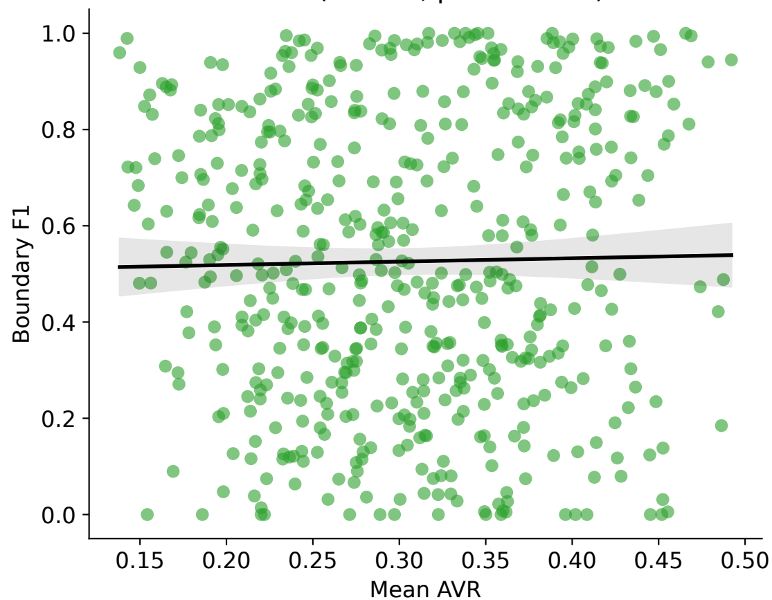
Swin ( r=0.02 , p=6.69e-01 )
