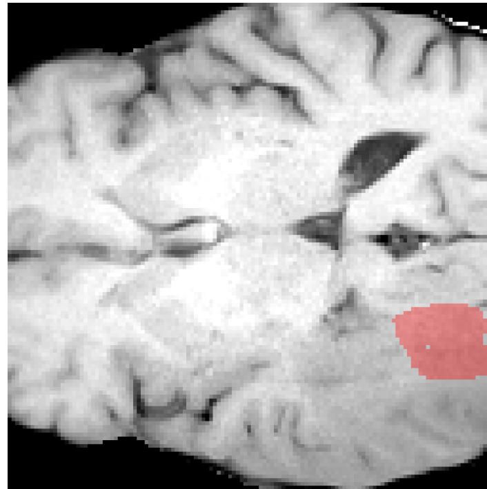
Baseline Prediction
