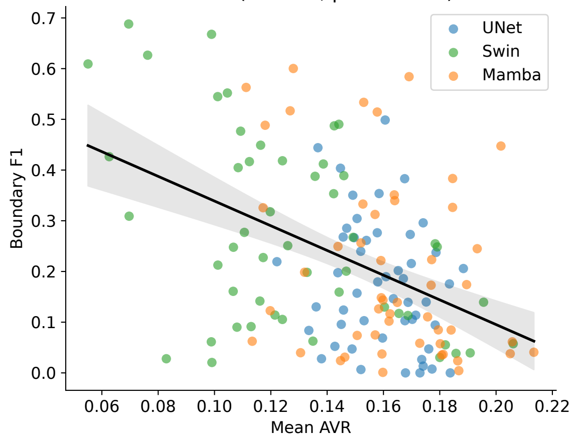
Pooled ( r=-0.44 , p=1.56e-08 )
