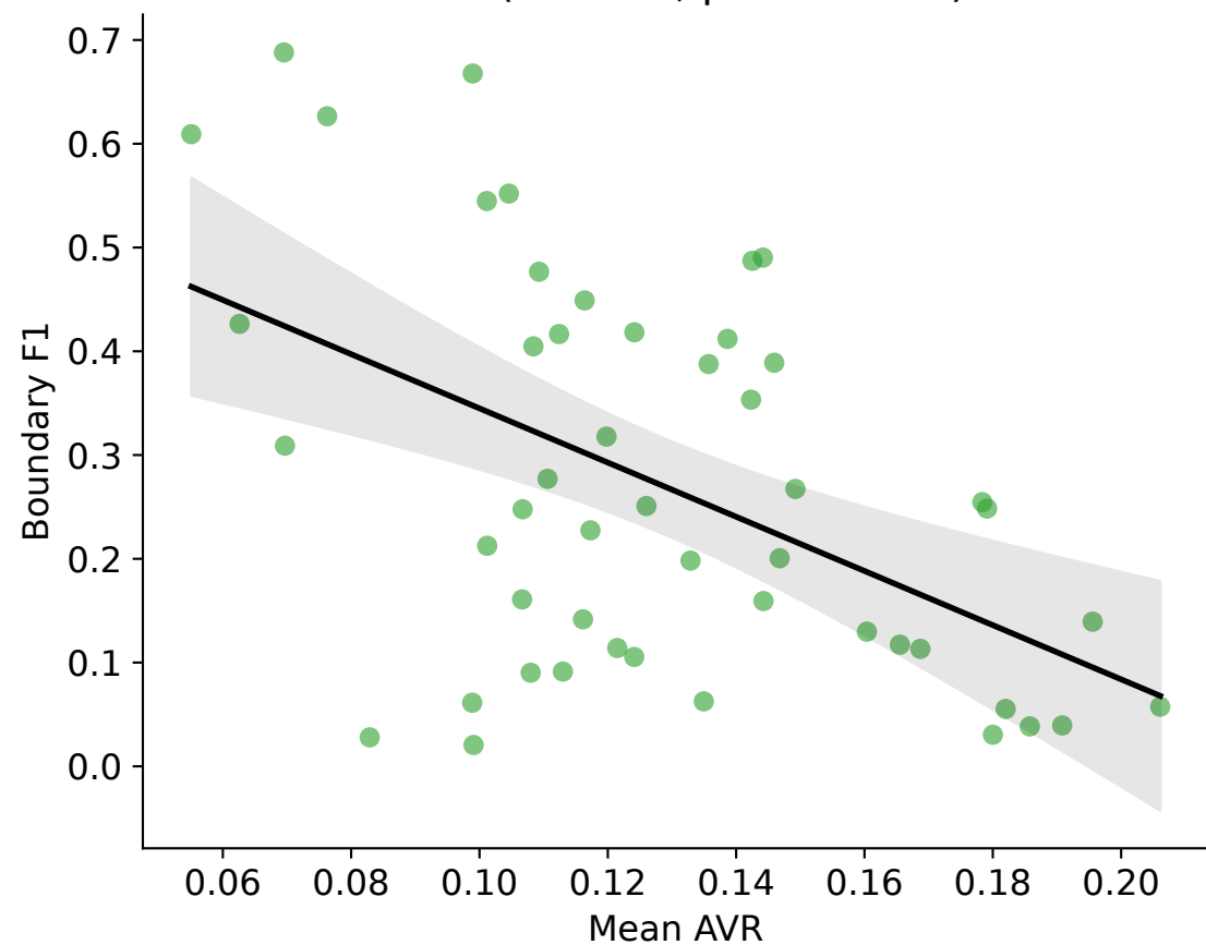
Pooled ( r=-0.44 , p=1.56e-08 )
