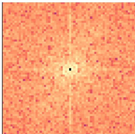
Mamba
